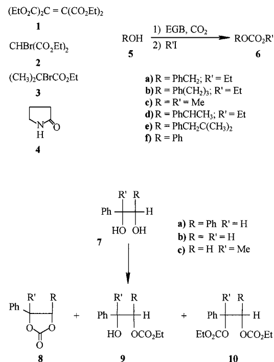
Scheme 1.
